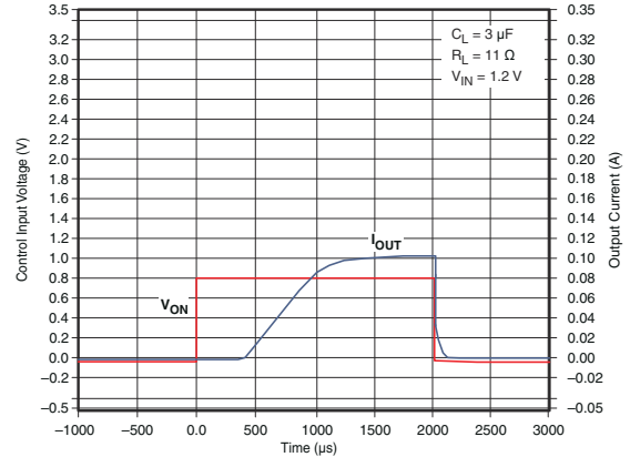
图 7-48. t_{ON} Response
