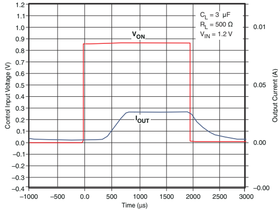
图 7-47. t_{ON} Response
